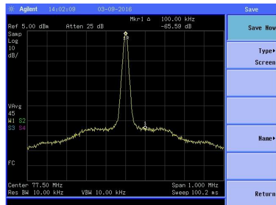
Figure 4-8 77.5 MHz tone, Span 1 MHz
